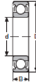
Two Shields ZZ
