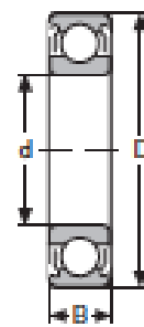
Two Shields ZZ
